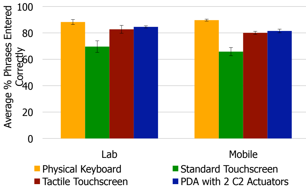
Figure 6-21: Average percentage of phrases entered correctly (with standard deviations).
