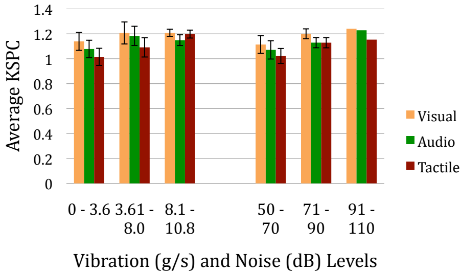
Figure 6-42: Average KSPC for vibration and noise level sets (with standard deviations).
