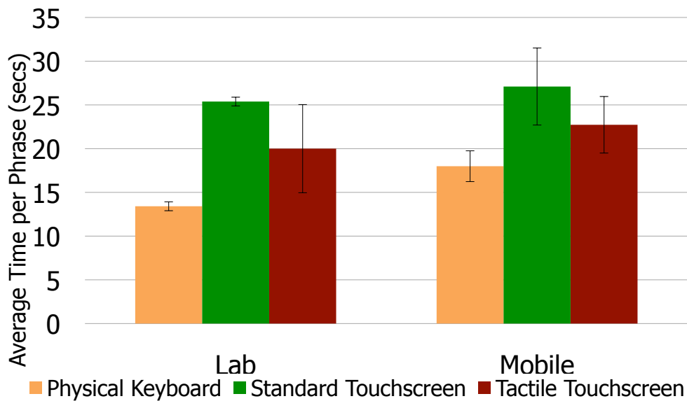
Figure 6-13: Average time per phrase entered in seconds (with standard deviations).
