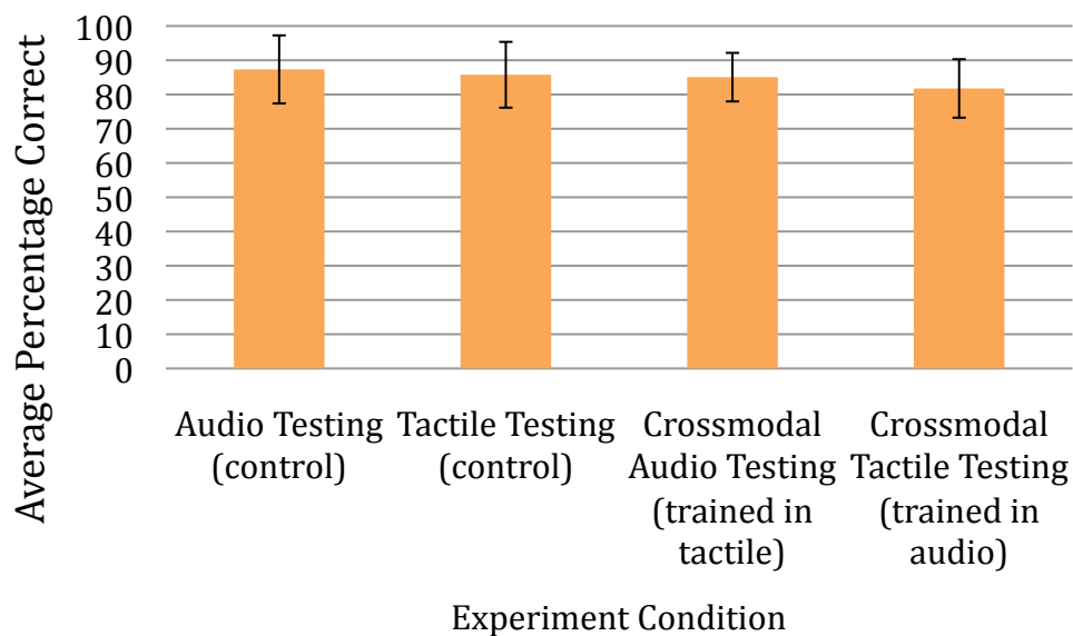
Figure 5-13: Average percentage of recognition rates during testing (with standard deviations).
