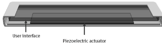
Figure 2-5: Touchscreen device with integrated piezo-electric actuator.
