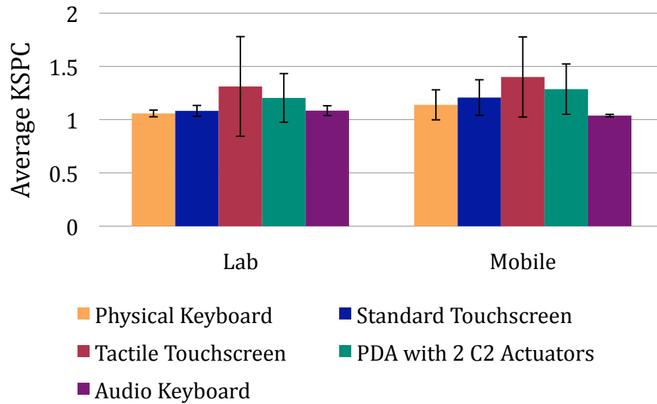
Figure 6-34: Average keystrokes per character (with standard deviations).
