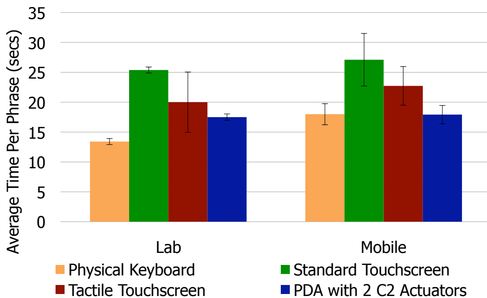
Figure 6-25: Average time per phrase in seconds (with standard deviations).
