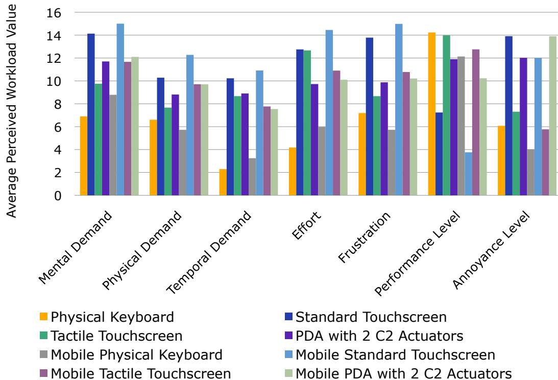
Figure 6-29: NASA TLX Scores Compared with Experiment 4a(i).
