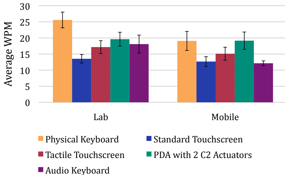
Figure 6-36: The average words per minute for each keyboard type along with static and mobile settings (with standard deviations).
