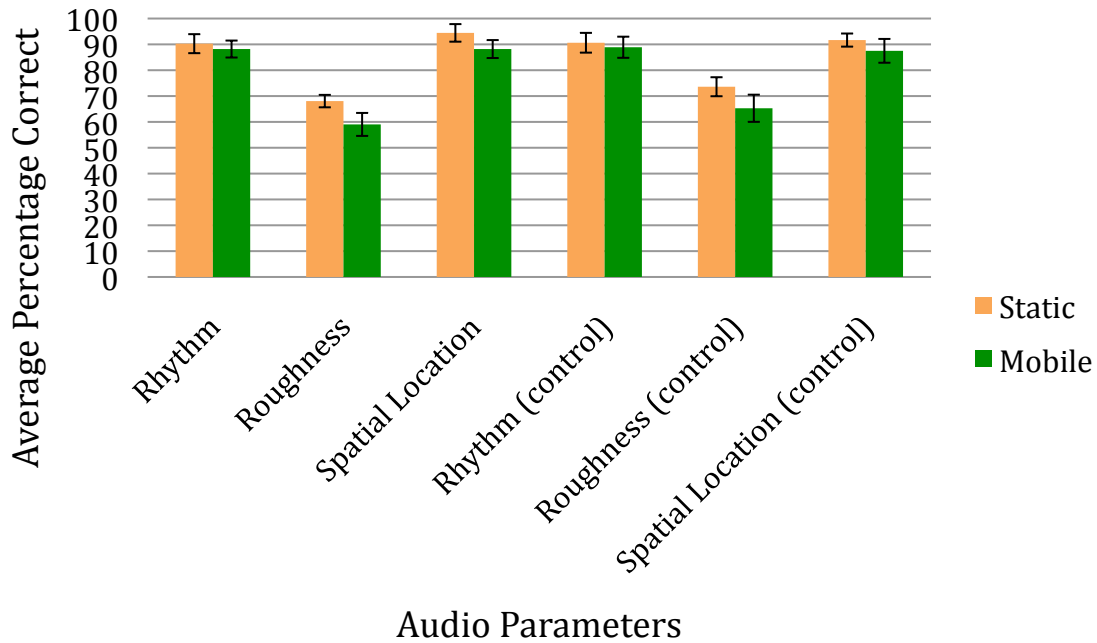
Figure 5-19: Average percentage of correct responses in each audio parameter (with standard deviations).
