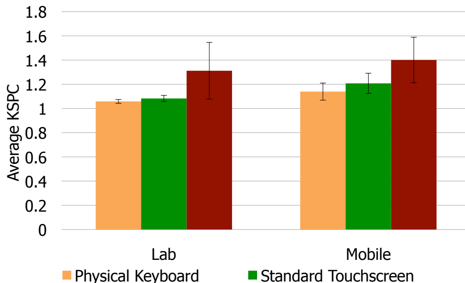
Figure 6-11: Average KSPC for each setting and keyboard type (with standard deviations).
