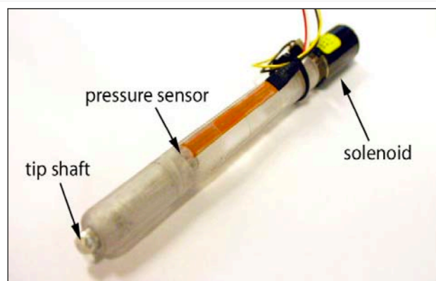
Figure 2-7: Haptic Pen Prototype.
