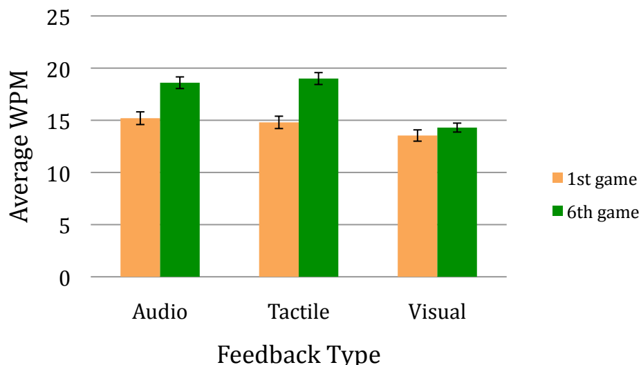
Figure 7-13: Average WPM for each feedback type at the beginning and end of each condition (with standard deviations).
