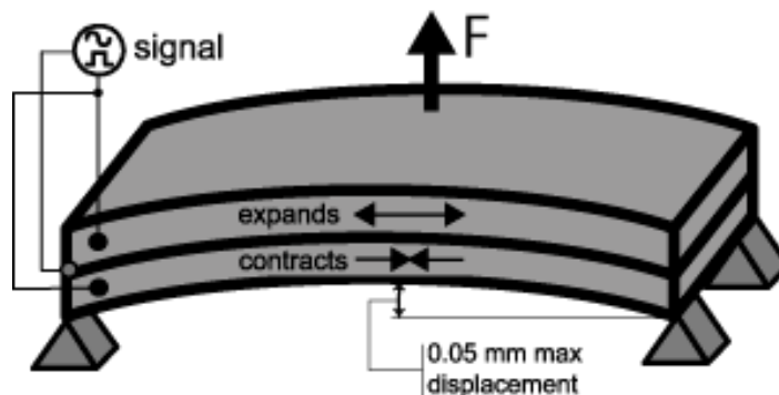
Figure 2-9: Piezo-electric bending motor actuator used in TouchEngine 8 .
