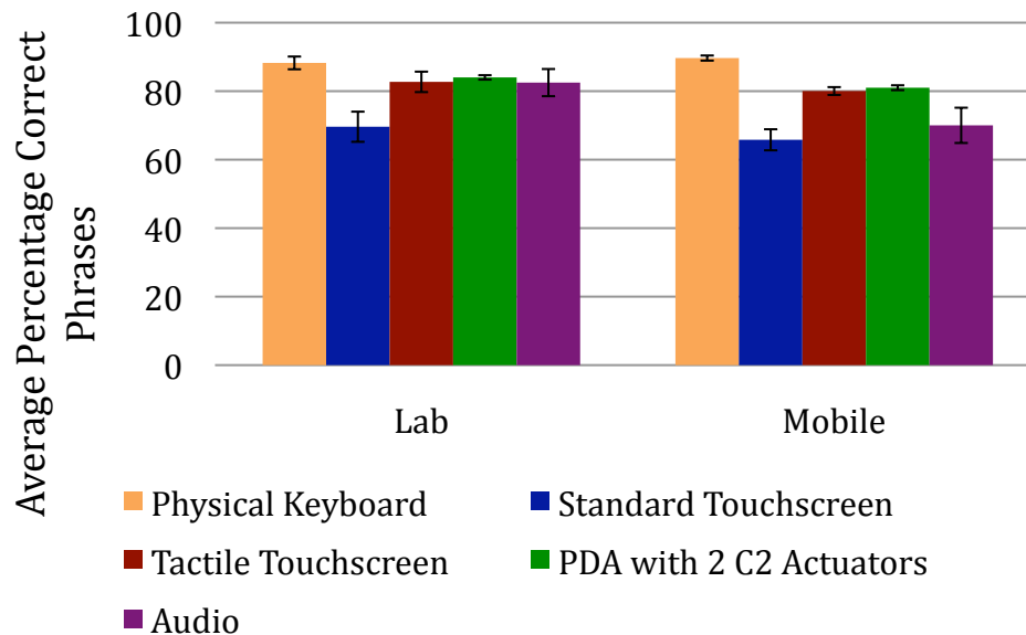
Figure 6-32: Average percentage of phrases entered correctly (with standard deviations).
