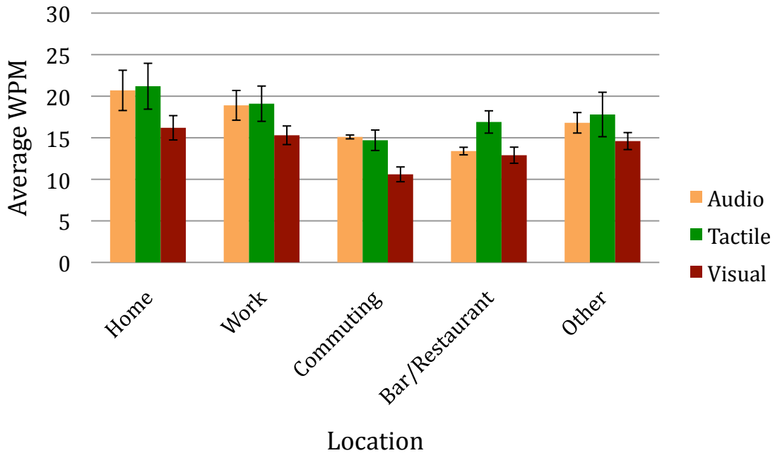
Figure 7-17: Average WPM for each modality per location (with standard deviations).
