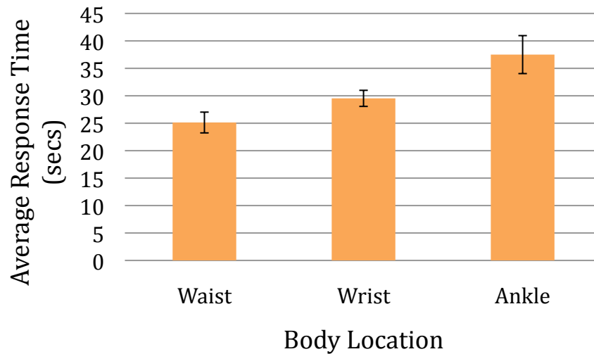
Figure 4-43: Average response time in seconds for each body location when mobile (with standard deviations).
