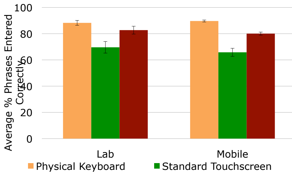
Figure 6-9: Average percentage of phrases entered correctly (with standard deviations).
