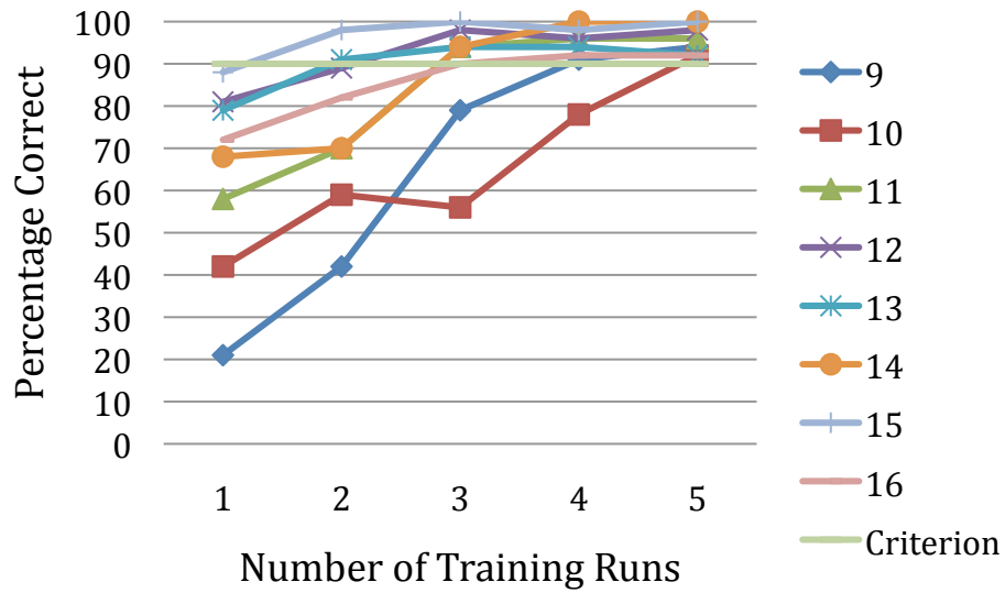
Figure 5-11: Learning curves for tactile training.
