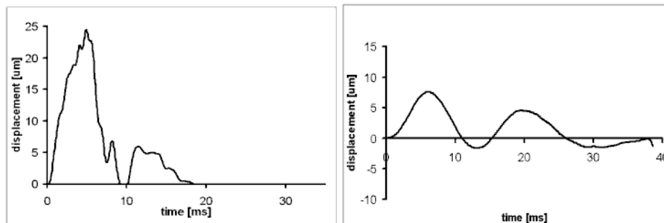
Figure 7-3: Example piezo-electric and vibrotactile output.
