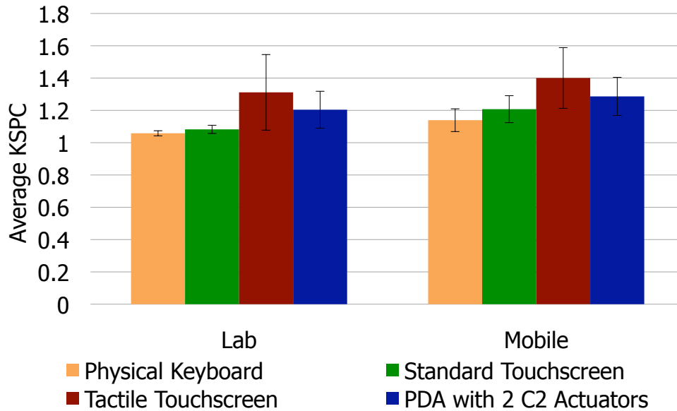
Figure 6-23: Average keystrokes per character (with standard deviations).
