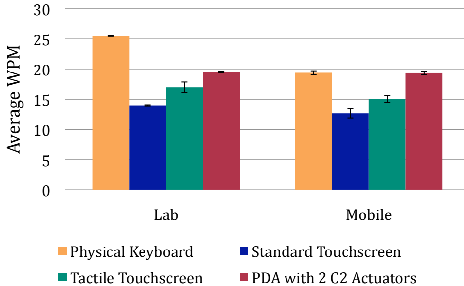
Figure 6-27: Average WPM for each keyboard type in the lab and mobile settings (with standard deviations).
