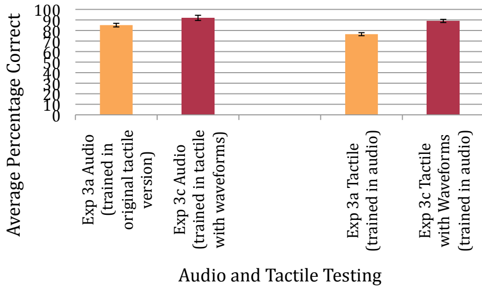
Figure 5-27: Average percentage correct in original experiment and follow-up experiment using tactile waveforms (with standard deviations).
