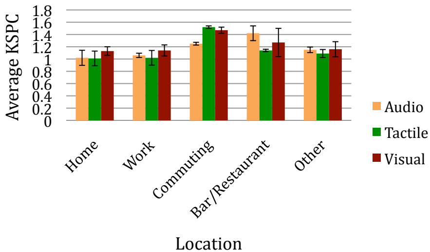
Figure 7-19: Average KSPC for each modality at each location (with standard deviations).
