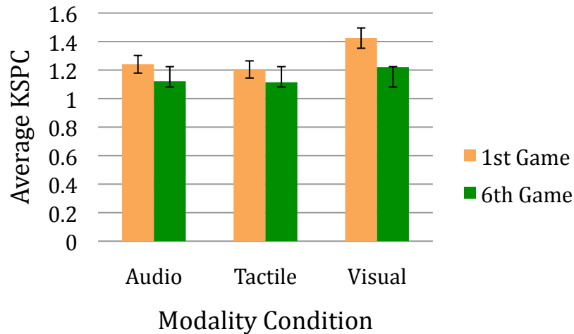
Figure 7-15: Average KSPC for each modality condition from first to last CrossTrainer games (with standard deviations).
