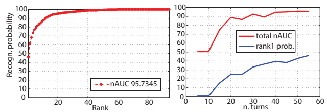
Figure 4. (left) Global CMC Curve; (right) nAUC and rank1 probability varying the number of turns.
