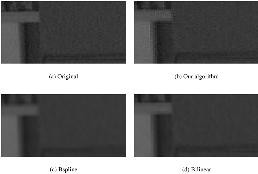
Figure 6: Samples taken from the frame shown in Figure 5. The algorithm convincingly synthesises speckle on the concrete wall but leaves the white wall in the background speckle free.
