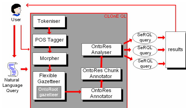
Figure 3: CLoNE Query Language Application
