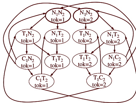
Figure 1: Kripke structure for 2 process mutual exclusion
