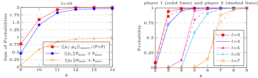
Fig. 2: Robot coordination: \langle\langle p_1:p_2 \rangle\rangle_{\max=?} (P[\mathbf{F}^{\leq k} \text{goal}_1] + P[\mathbf{F}^{\leq k} \text{goal}_2]) ( q=0.1 )
