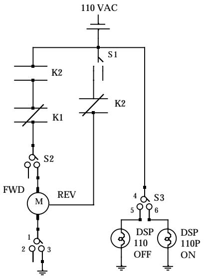
FIGURE 7.10-4: EXAMPLES OF CATEGORIES OF SNEAK CIRCUITS
