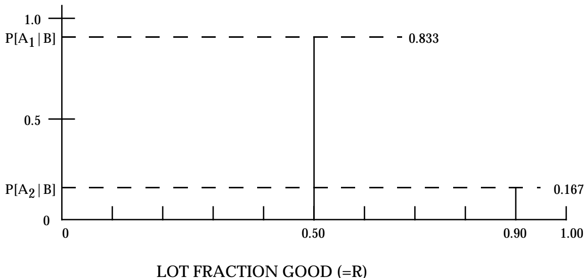
FIGURE 5.5-2: SIMPLE POSTERIOR DISTRIBUTION
