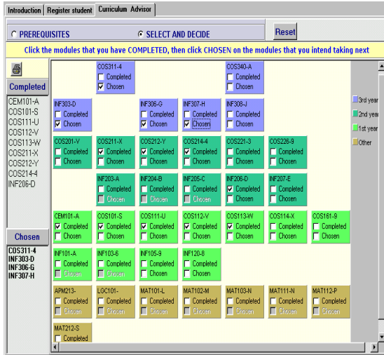
Figure 3: Bottom-Up Approach
