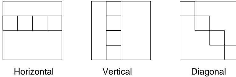
Figure 2: Implied Templates
