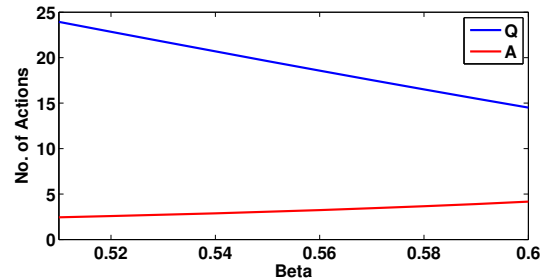
Figure 4: Plot of \mathbf{A}^* and \mathbf{Q}^* as \beta changes.
