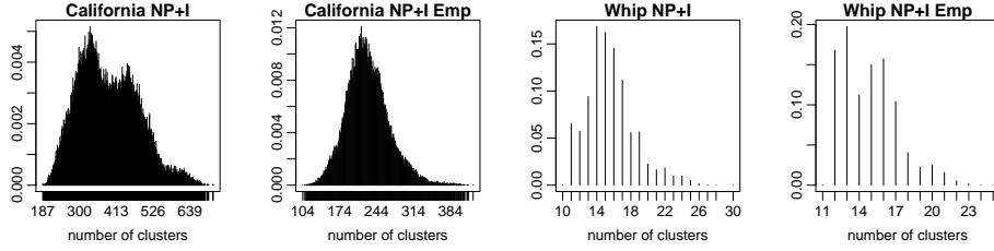
FIG 2. Posterior distribution of the number of clusters for the California and WHIP tables when using the (NP+I) and (NP+I) Emp models.
