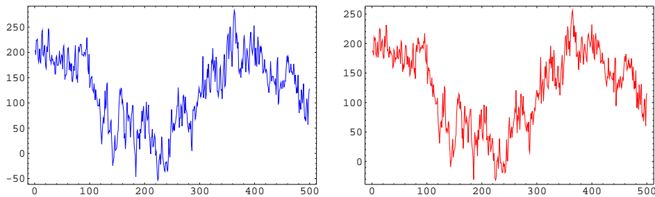
Figure 3: Data Set Paris-14E Parc Montsouris. The original target data and the results yielded by SVM (model order = 10) are shown on the left and the right respectively.
