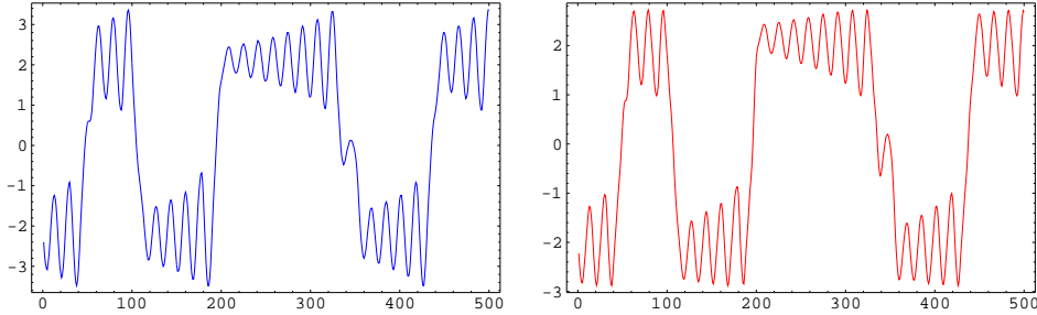
Figure 4: Chua Time Series. The original target data and the results yielded by SVM (model order = 5) are shown on the left and the right respectively.
