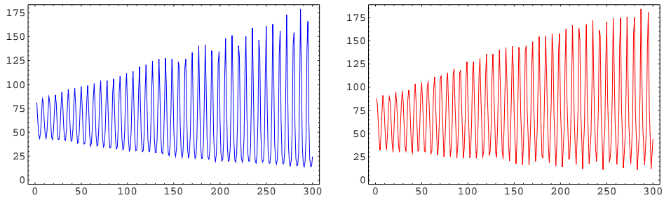
Figure 2: Data Set A of Santa Fe Competition. The original target data and the results yielded by SVM (model order = 4) are shown on the left and the right respectively.
