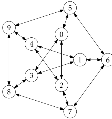
Figure 12.7: An example graph.
