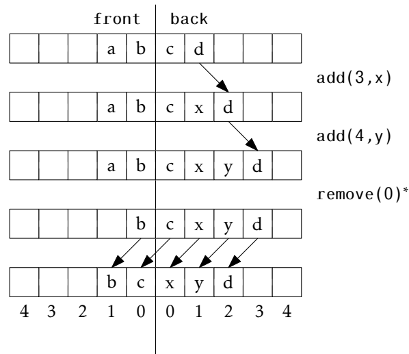
Figure 2.4: A sequence of \text{add}(i, x) and \text{remove}(i) operations on a DualArrayDeque . Arrows denote elements being copied. Operations that result in a rebalancing by balance() are marked with an asterisk.
