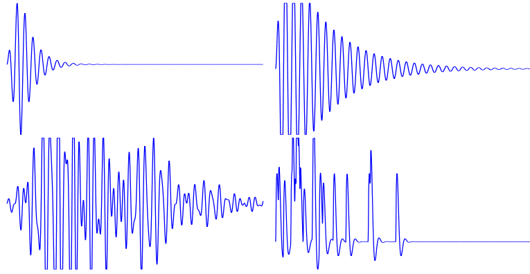
Figure 4: Four different vibrotactile waveform types. Left-to-right, top-to-bottom: standard “light ball” impact; heavy, ringing impact; liquid sloshing; gritty, particulate impact. All of these have energy concentrated around the 250Hz band.
