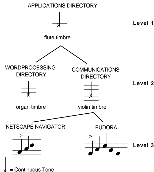
Figure 1: A hierarchy of earcons representing a family of applications. The '>' symbols over a note indicate stress or accent.
