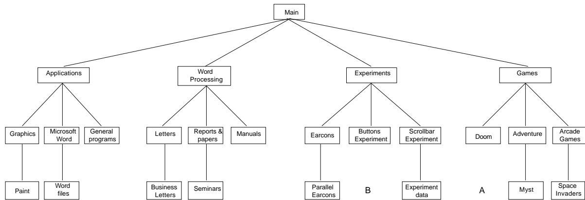
Figure 3: The file-system hierarchy used in the experiment. A and B show the two new earcons presented to participants during testing.
