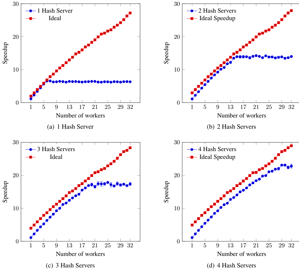
Figure 19. GAP5 Harada-Norton Orbit Speedups (NUMA)
