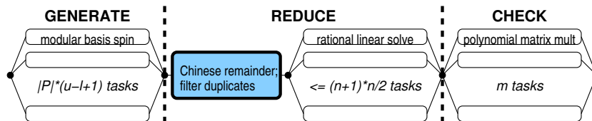
Figure 21. Structure of parallel algorithm for computing Q .
