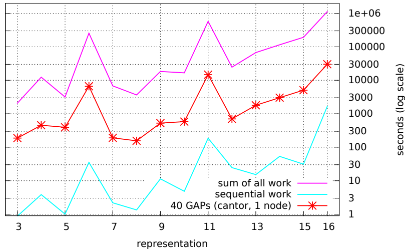
Figure 22. SymGridPar2 Computing Hecke Algebra Q Runtimes (NUMA)
