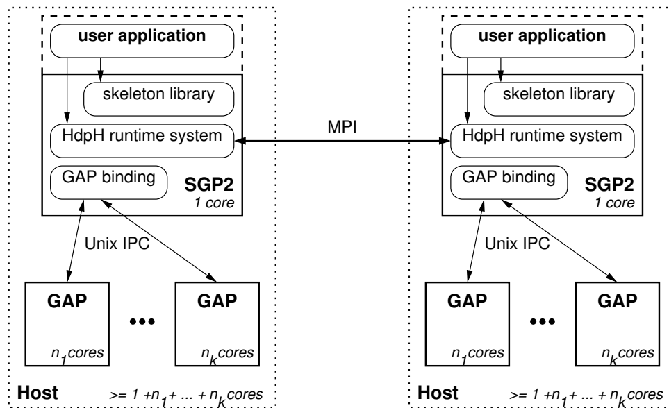
Figure 5. SymGridPar2 Architecture.
