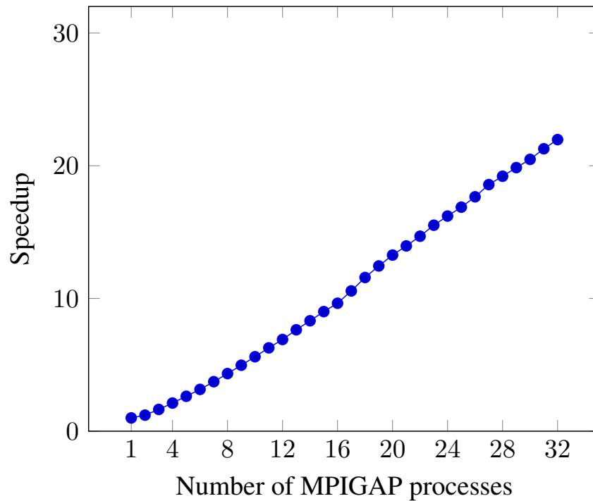
Figure 12. MPIGAP SumEuler Speedups (Beowulf Cluster).
