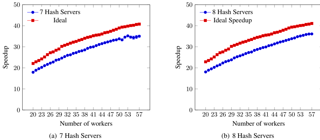
Figure 20. GAP5 Harada-Norton Orbit Speedups with 7 or 8 Hash Servers (NUMA)
