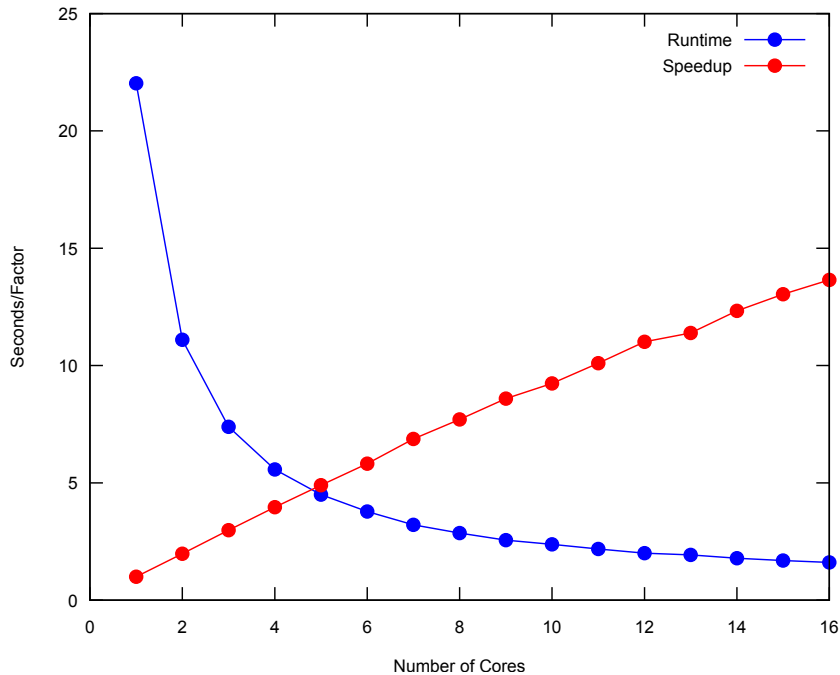
Figure 11. GAP 5 SumEuler Runtimes and Speedups (Multicore).
