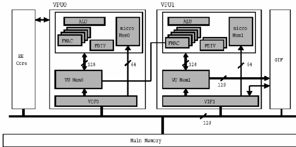
FIGURE 4.1. The architecture of the PS/2 processor. The EE core incorporates a SIMD unit analogous to that shown in Figure 3.1.
