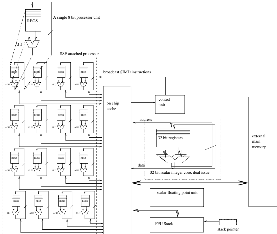
FIGURE 3.1. Outline of the Intel P4 architecture showing the incorporated Streaming SIMD unit.
