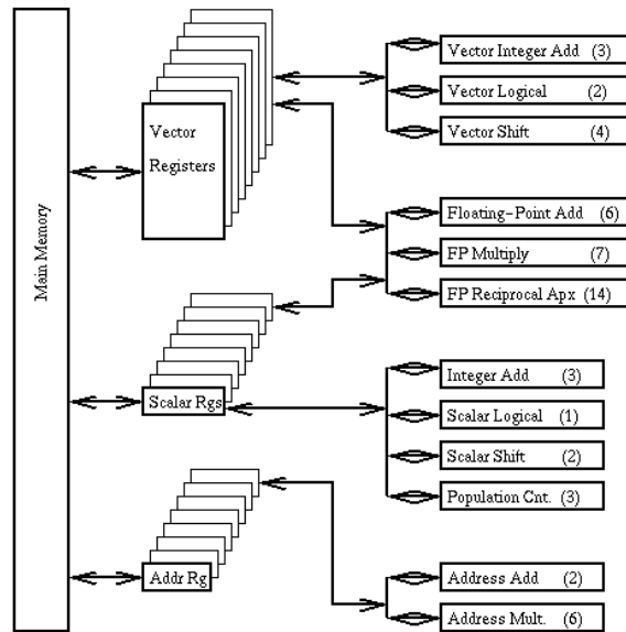
FIGURE 2.1. Basic Cray 1 architecture showing vector registers.
