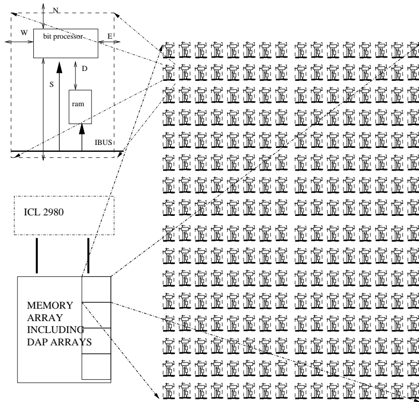
FIGURE 2.2. The ICL DAP showing a bit processor and 16th of the array of 4096 such processors
