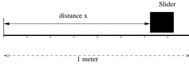
FIGURE 1. An analogue representation of a real number using a physical version of the real number line.
