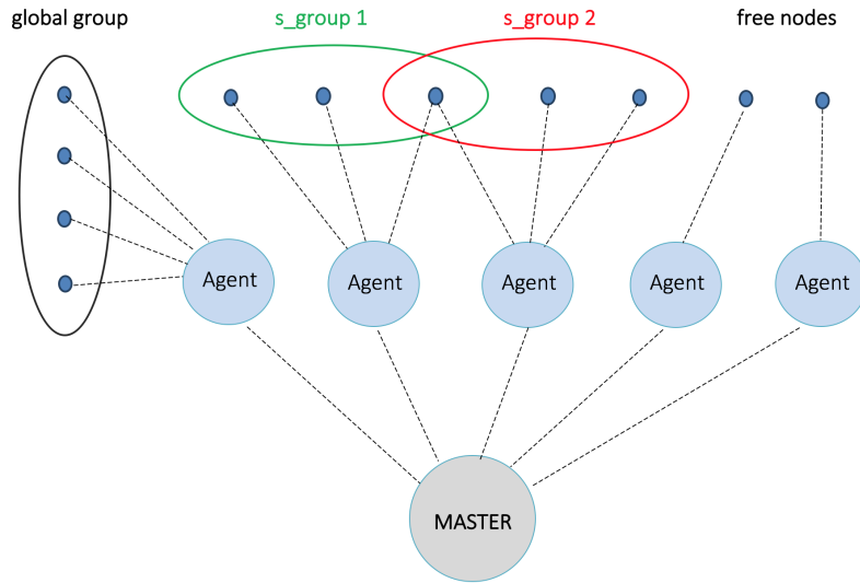
Figure 26: SD-Mon architecture.
