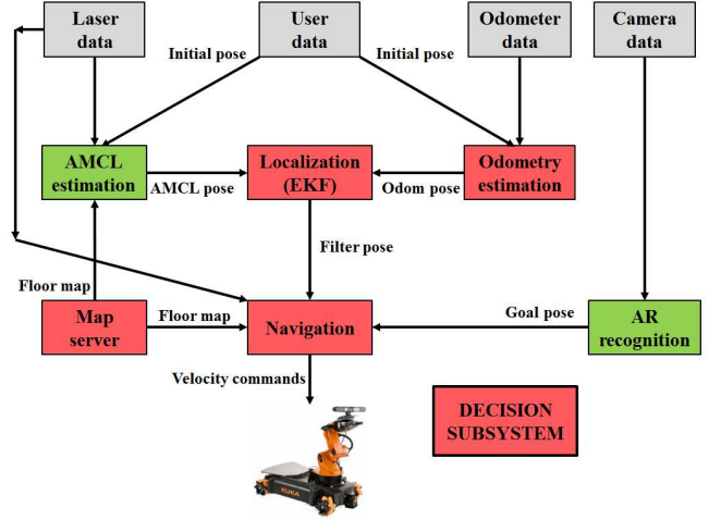
Fig. 3. System flow diagram: ROS nodes (providing data [grey], critical [red], and migratable [green]) and connections.
