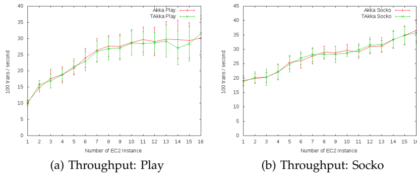
Figure 14: Throughput Benchmarks
